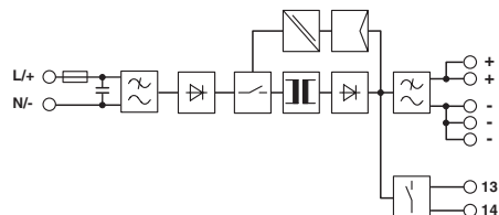
Block diagram
